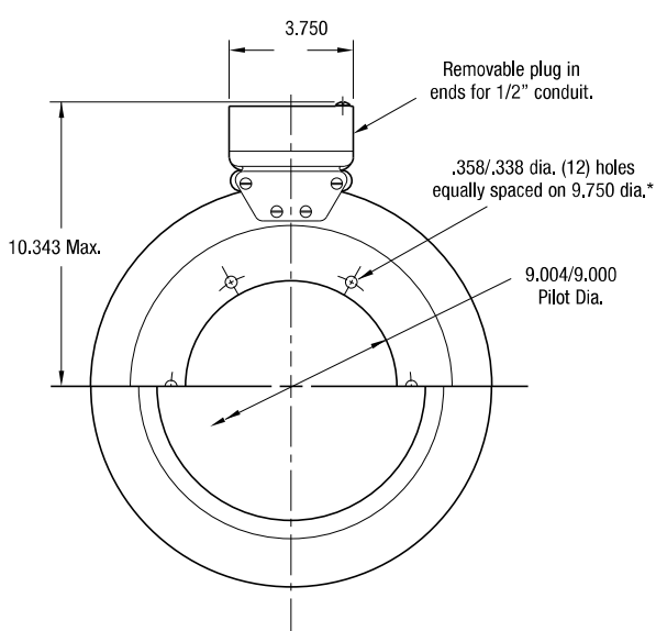
MAGNET VIEW
