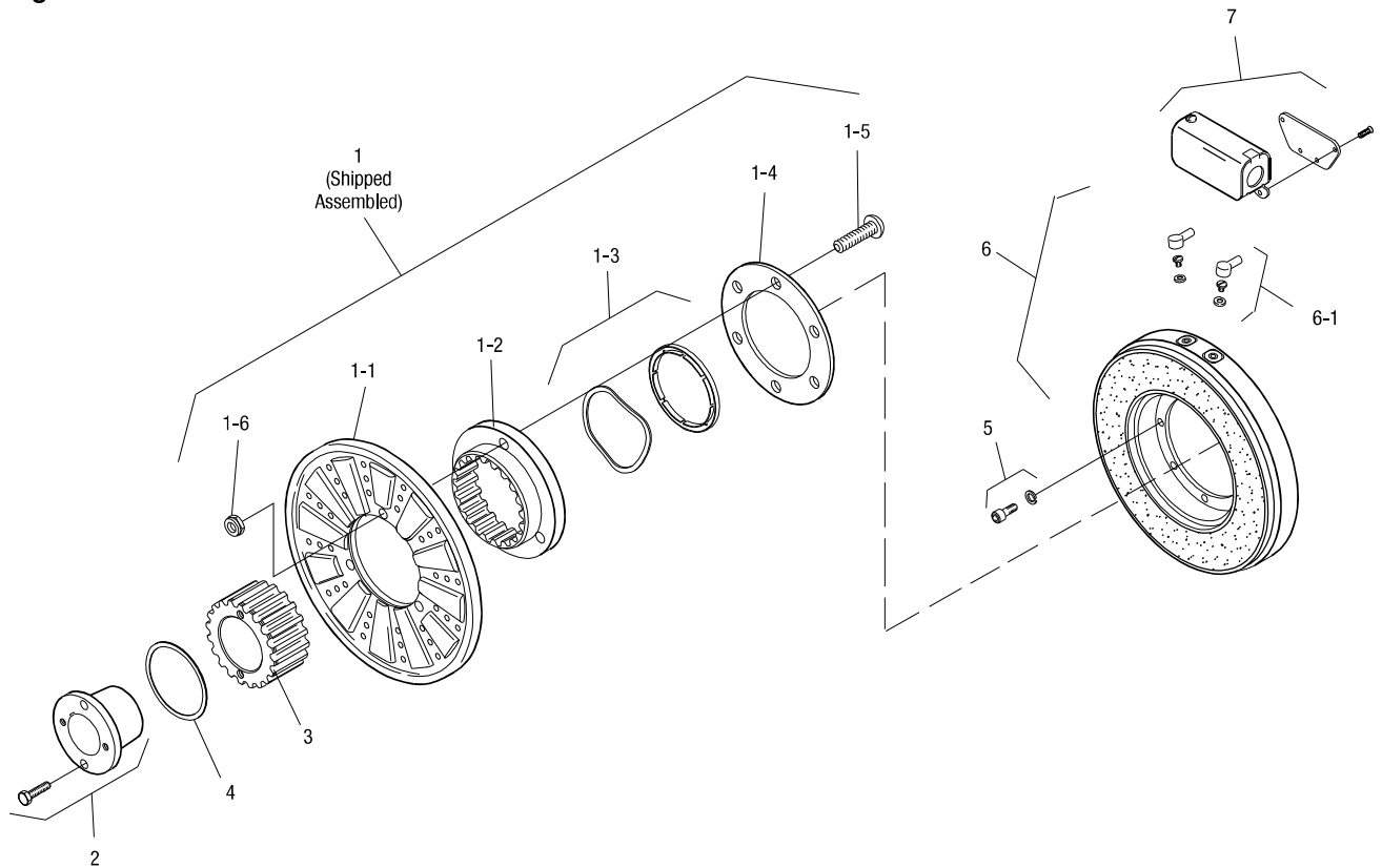
Drawing I-25634
