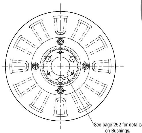
ARMATURE VIEW
